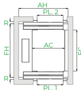
2 Entrances (open through)
